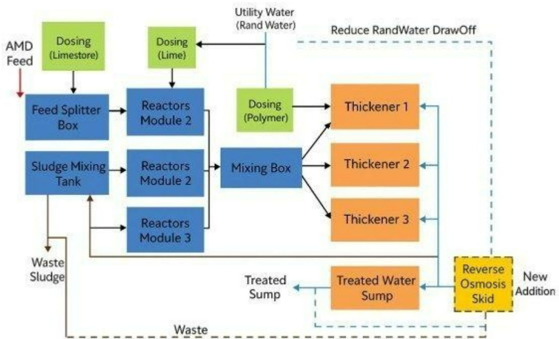
Figure 3-2: Schematic representation of the AMD treatment process
